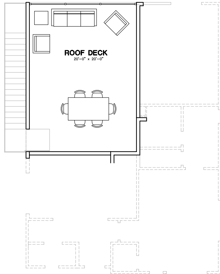
ROOFTOP DECK OPTION
