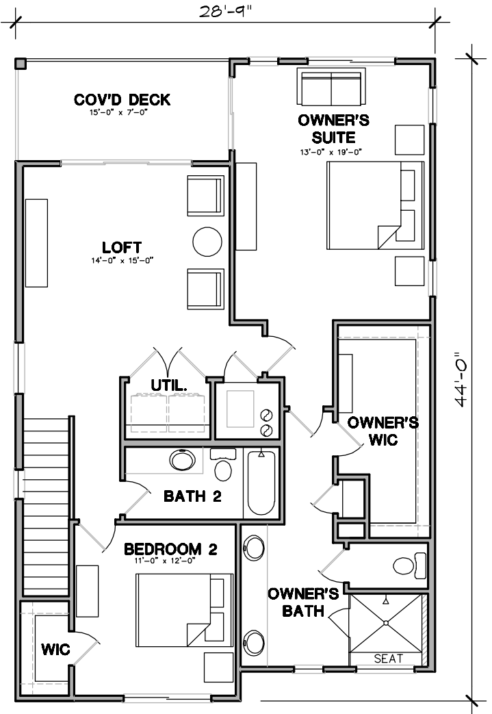
THIRD LEVEL FLOOR PLAN
