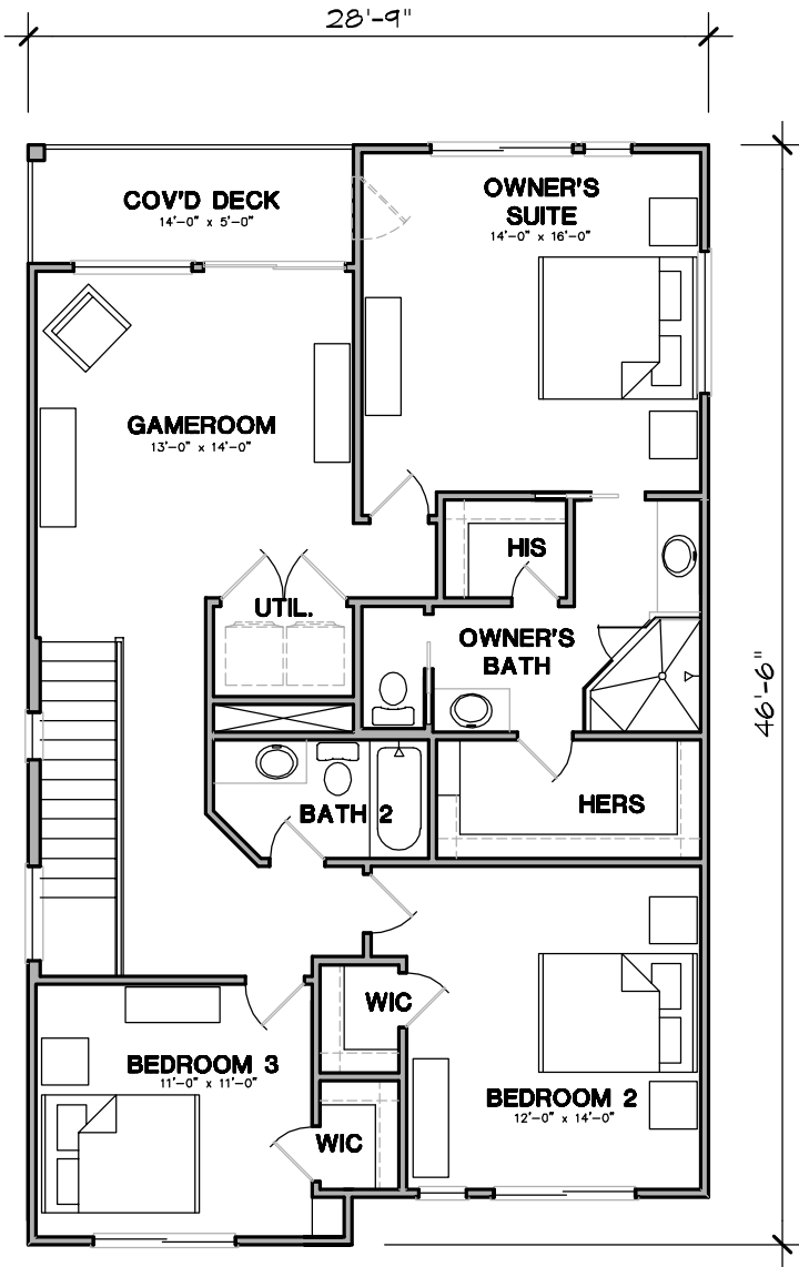
SECOND LEVEL FLOOR PLAN
