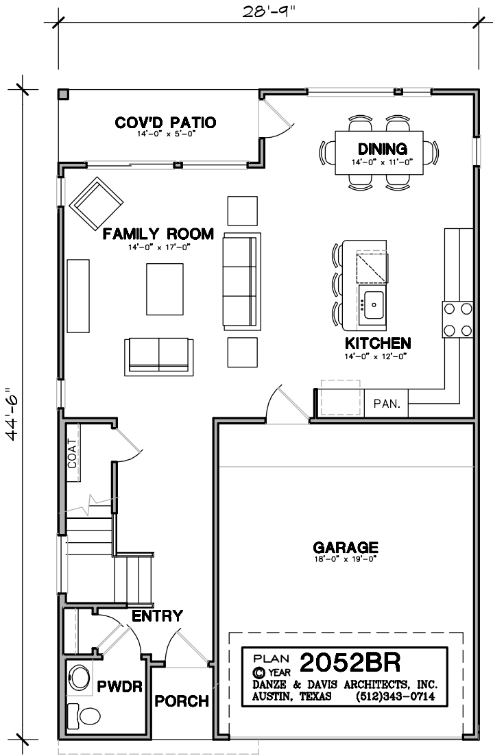
FIRST LEVEL FLOOR PLAN
