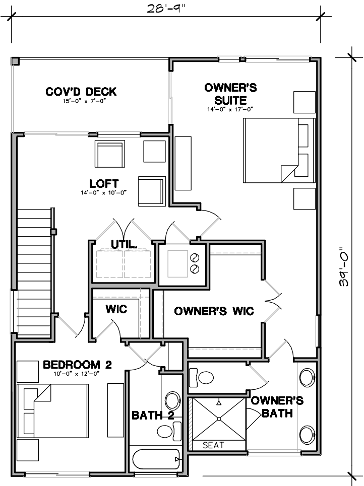
THIRD LEVEL FLOOR PLAN
